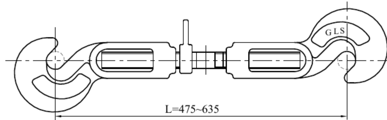
CE-B1/H Hook/Hook
